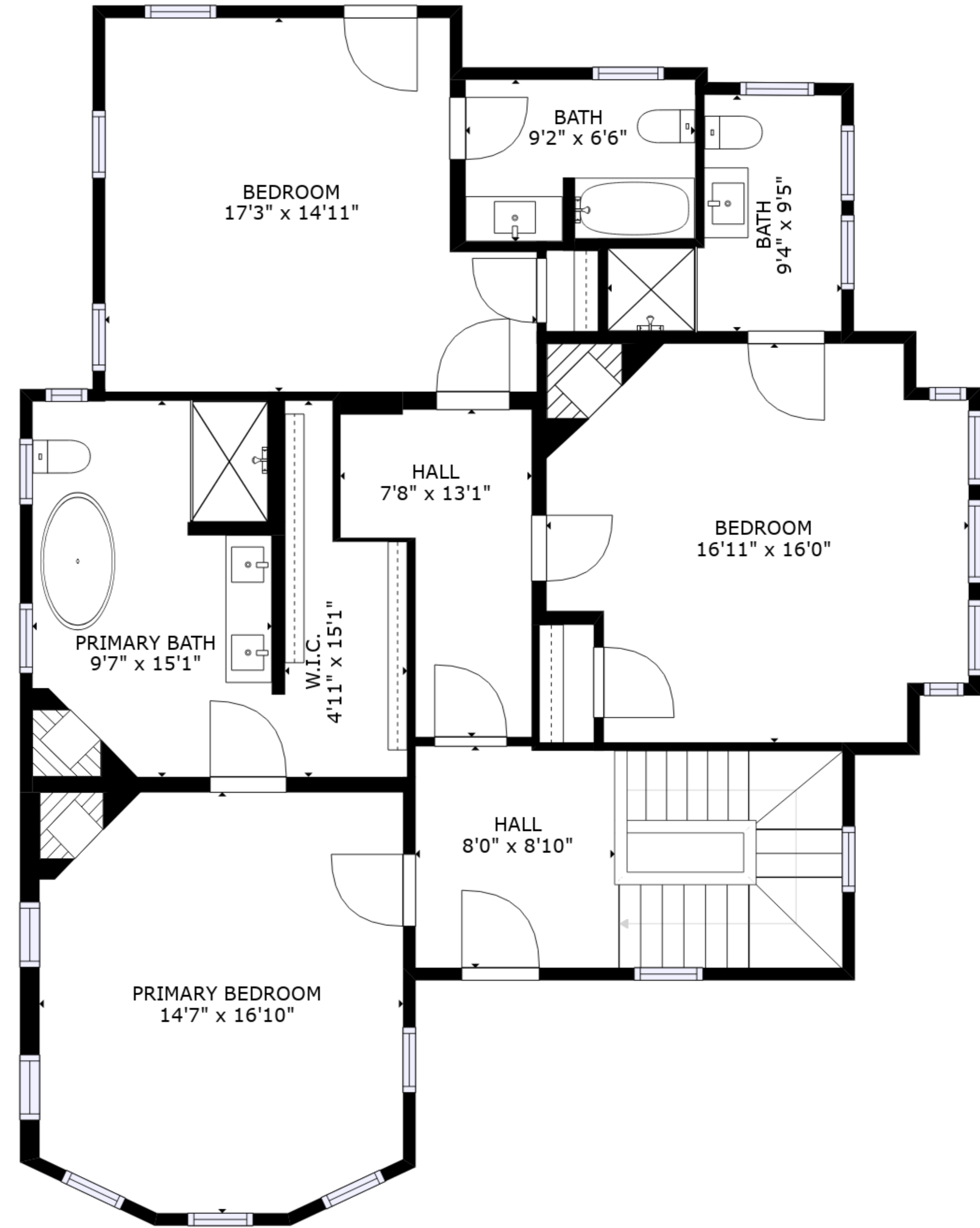
FLOOR 2
