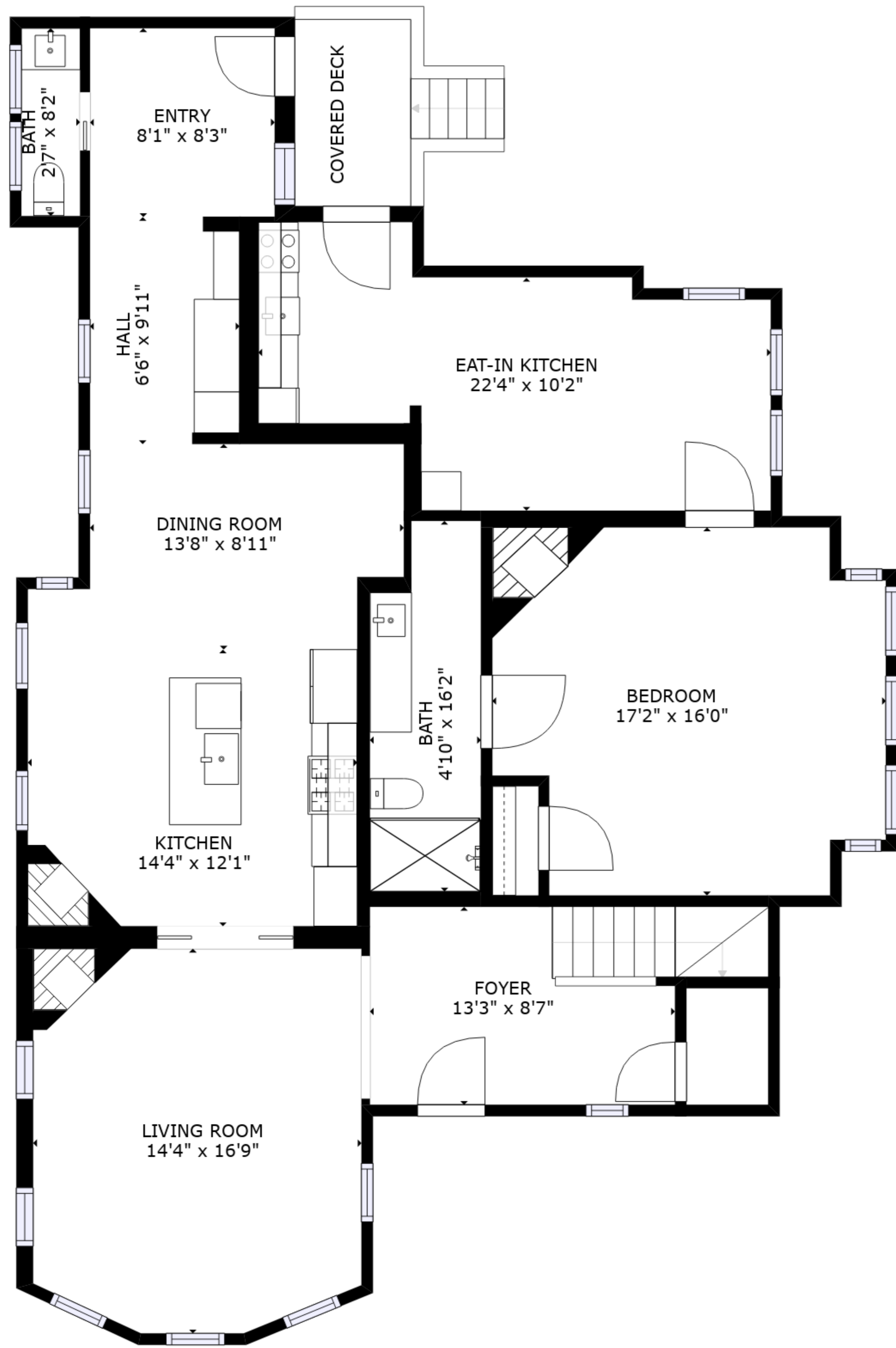
FLOOR 1
